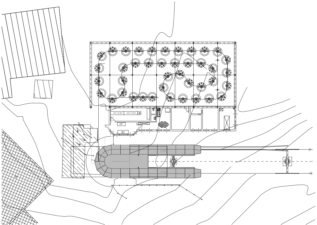
Lower station with parking facility - project
