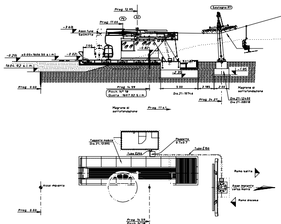
Lower station - project
