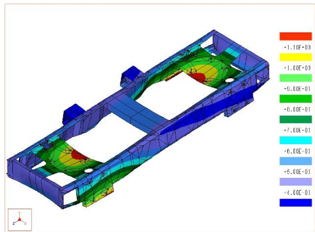
FEM - Model
